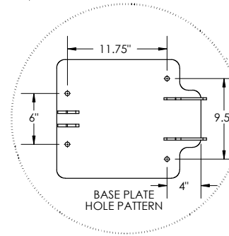
Top View (Retracted)
